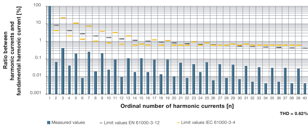
Harmonic currents at rated output SolarMax 4200S / 6000S ( R_{sc} = 33 )
